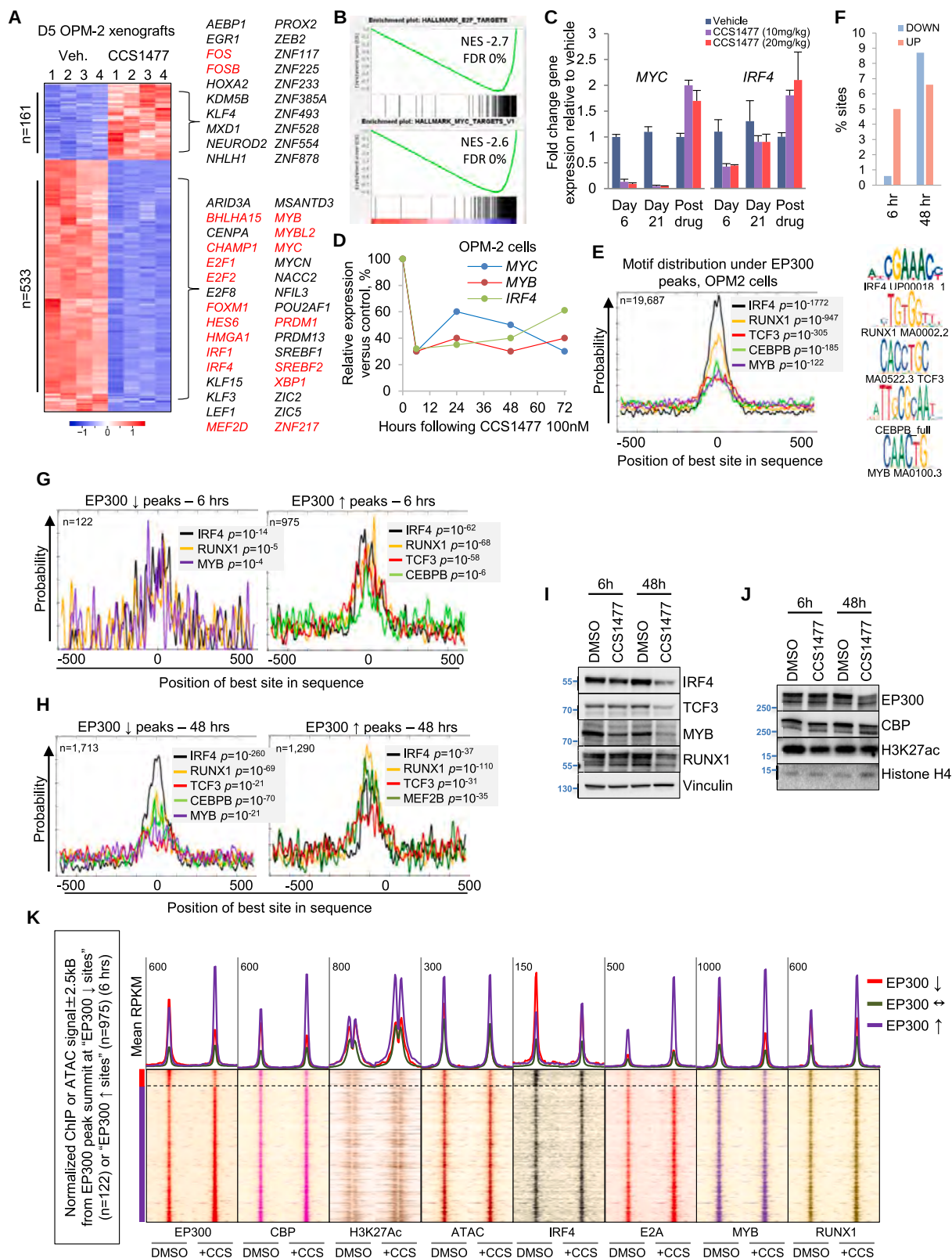
Figure 5. CCS1477 induces loss of EP300 from IRF4 and MYB-bound enhancers in myeloma cells
