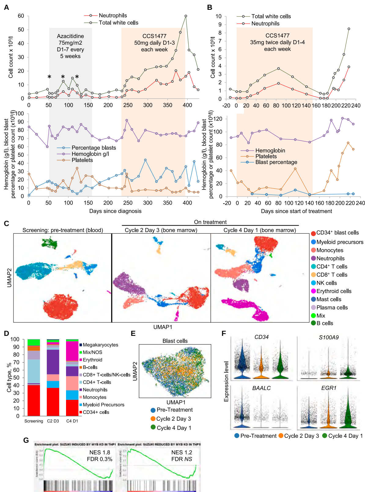
Figure 7. CCS1477-induced granulocytic differentiation responses in poor prognosis patients with AML
