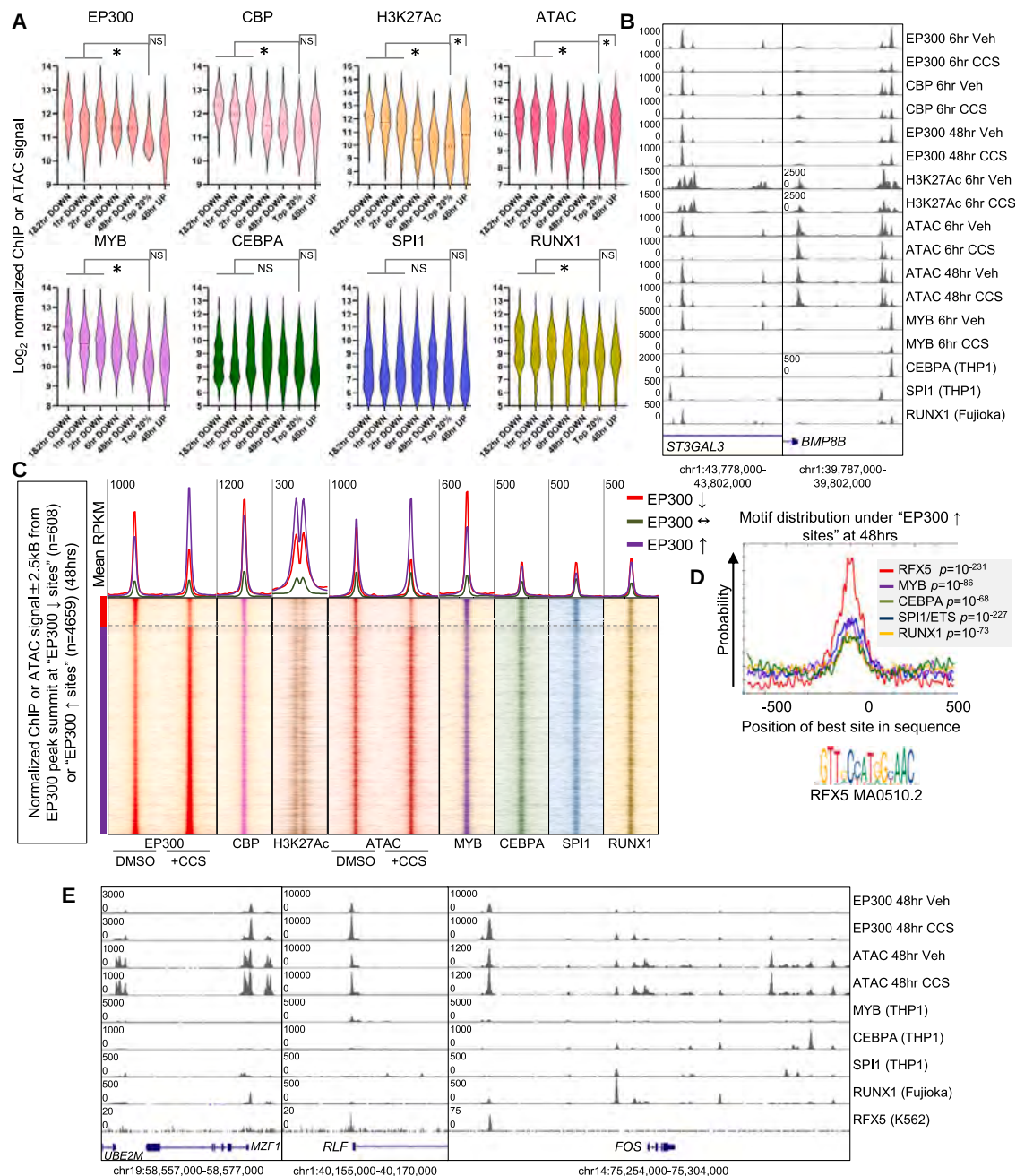
Figure 3. Redistribution of EP300-binding sites upon extended CCS1477 exposure in THP1 AML cells
