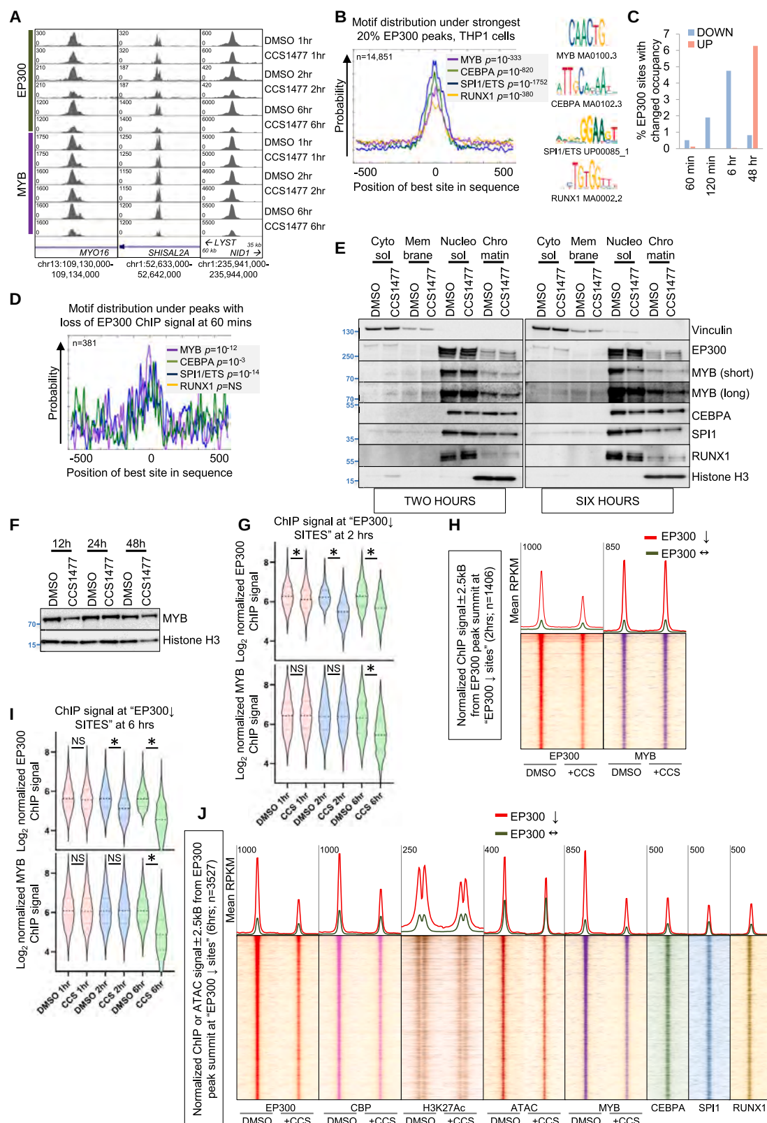
Figure 2. CCS1477 induces rapid but selective loss of EP300 from enhancers in THP1 AML cells
