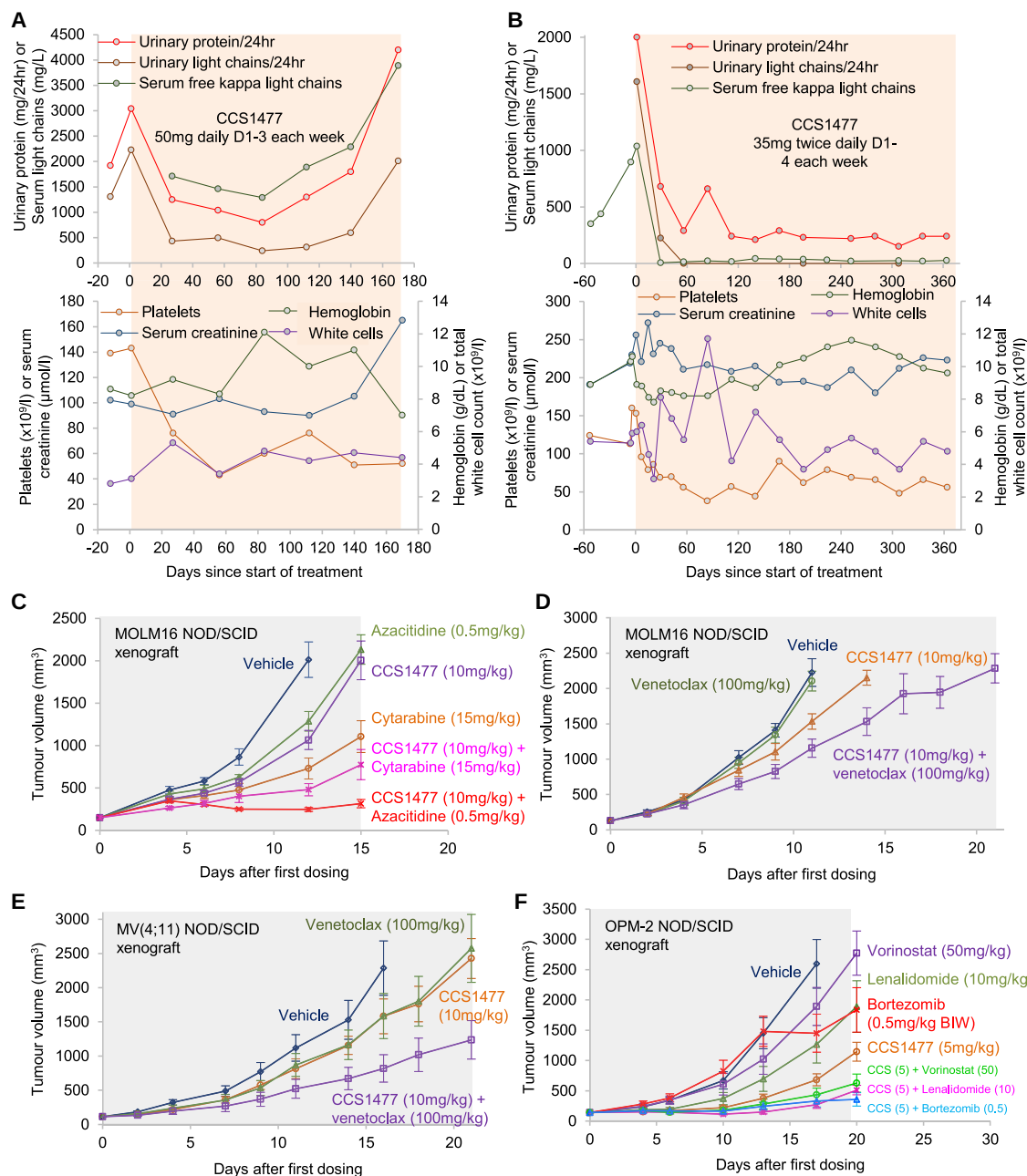
Figure 8. Responses in patients with heavily pre-treated myeloma and evaluation of combination therapy with standard-of-care agents (A) and (B) Exemplar disease and treatment response trajectories. Growth curves show mean + SEM tumor volume in xenograft experiments ( n = 5 mice/cohort) with (C), (D) MOLM16 AML cells, (E) MV(4; 11) AML cells, and (F) OPM-2 myeloma cells with CCS1477, the indicated standard-of-care agents, or a combination of the two. See also Figure S8 .
