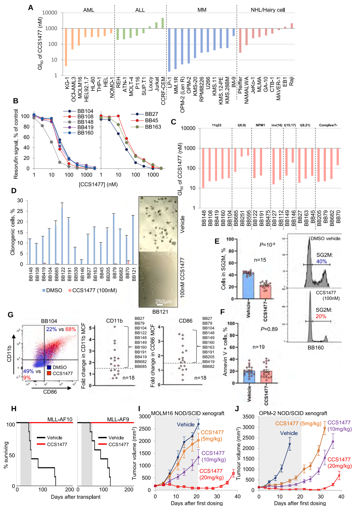
Figure 1. Sensitivity of hematologic malignancy cell lines, primary samples, and mouse models to CCS1477
