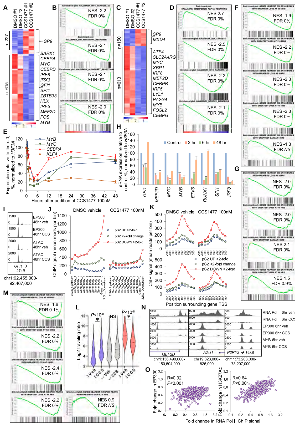
Figure 4. CCS1477-induced changes in EP300 occupancy alter enhancer activity and associated transcriptional program
