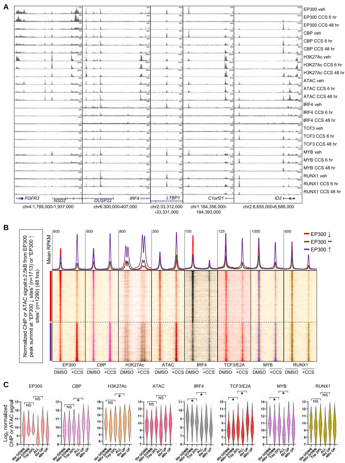
Figure 6. Longer CCS1477 treatment induces redistribution of EP300 in OPM-2 myeloma cells
